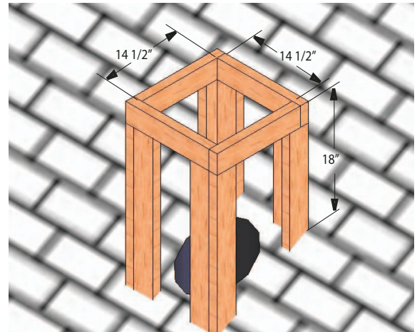
Figure 11. Chase box dimensions.
