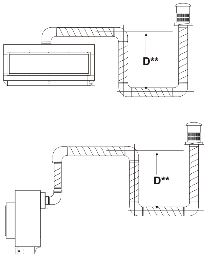
Figure 10b. Multi-Elbow with downward vent run, Top or Rear Vent, Roof mounted power vent.
