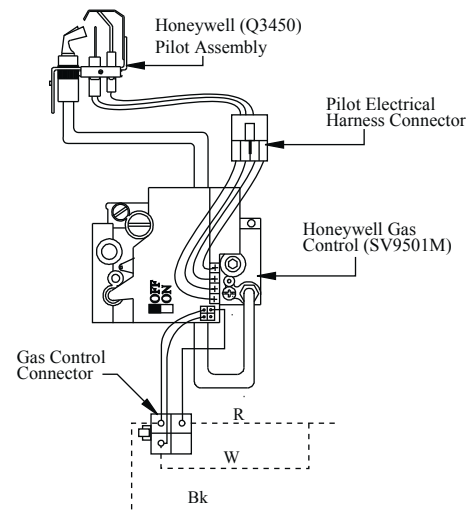
Figure 23. Gas valve.
