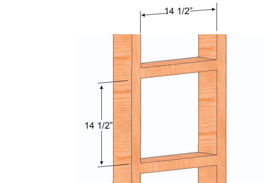
Figure 13. Frame dimensions.
