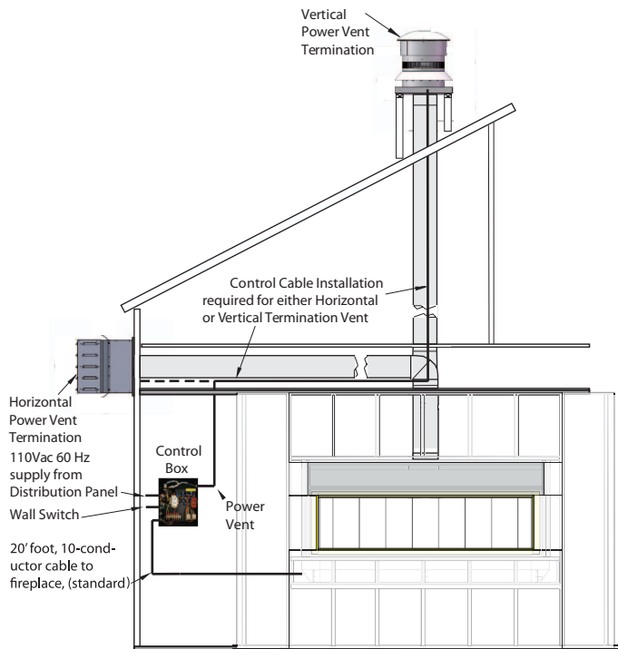
Figure 15. R320* / R420* Series Control Box / Power Vent Wire Routing Diagram
