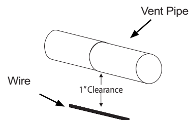
Figure 16a. Conduit and Wiring Clearances.
